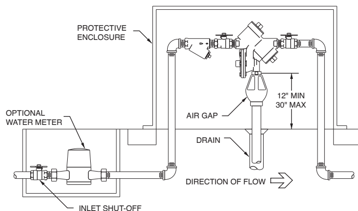
OUTDOOR INSTALLATION
